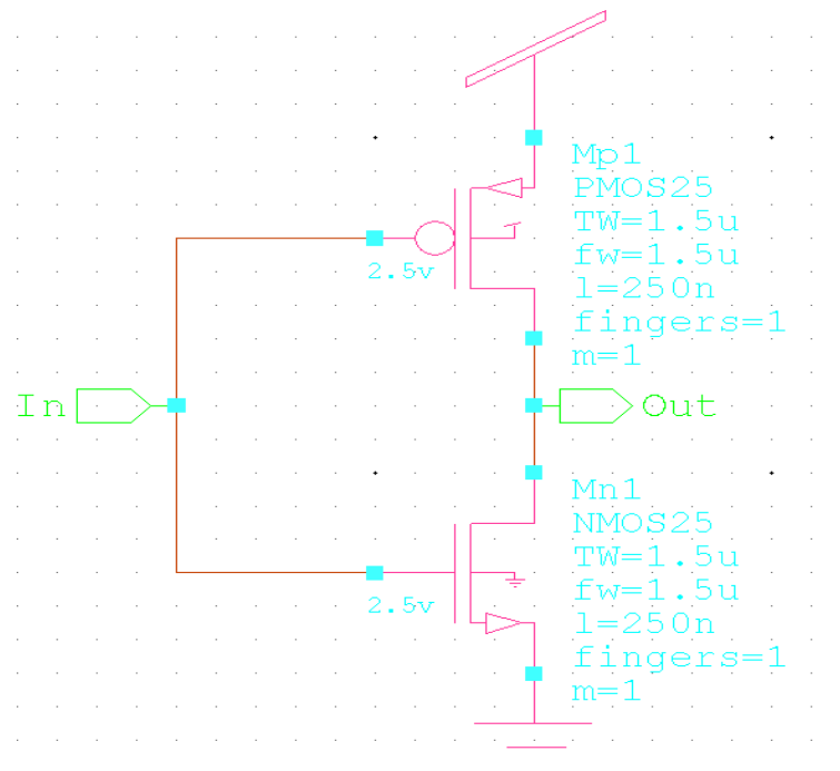
Fig3.2: INVERTER SCHEMATIC
