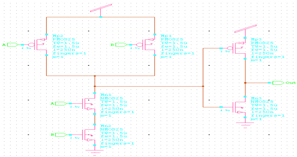
Fig3.4:ANDSCHMATIC
