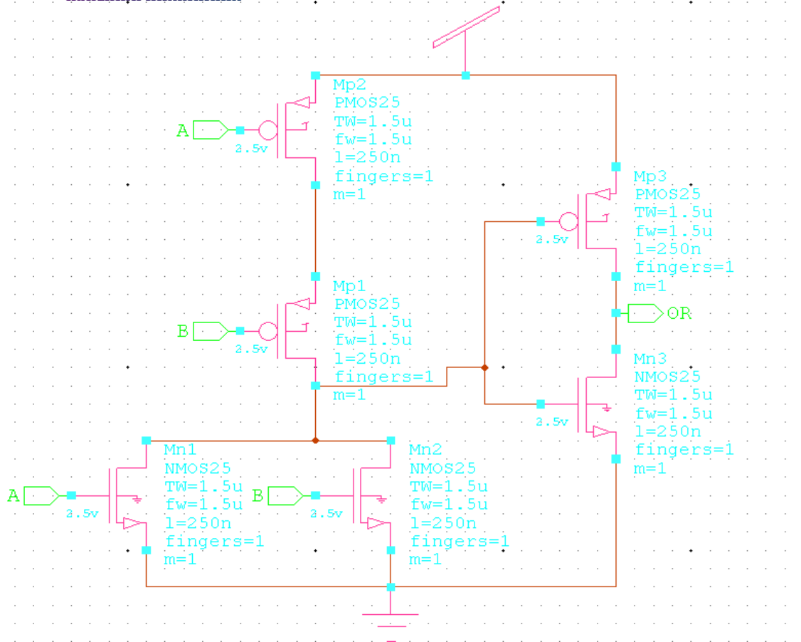
Fig3.5:ORSchematic
